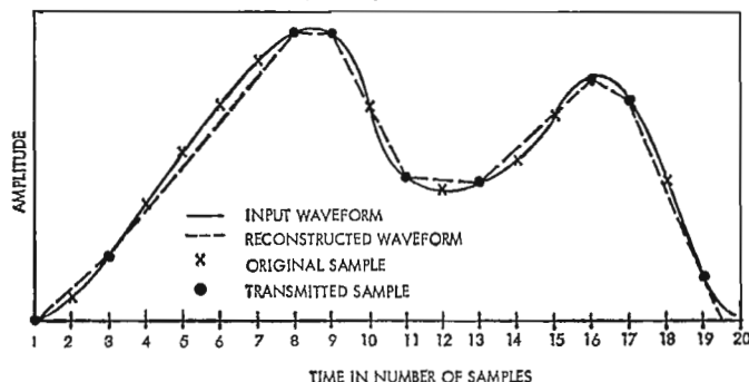
Fig. 4. In the first-order redundancy reduction method, waveform is reproduced by using straight-line approximations.
