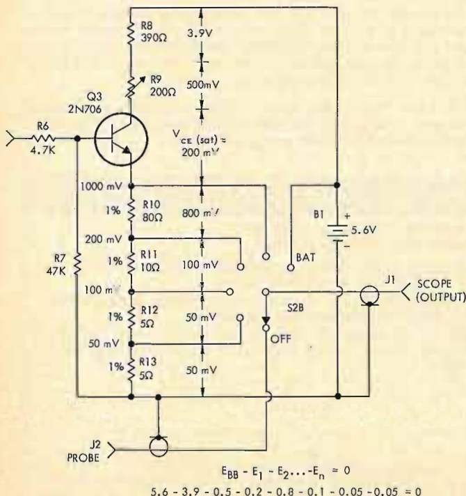
Fig. 1. Basic calibrator consists of 1% precision divider.
