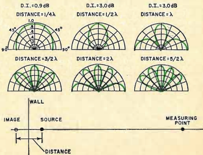
Fig. 5. Directivity patterns for speaker near wall. Vertical axes in polar charts (response in ratios) correspond to on-axis line below.
