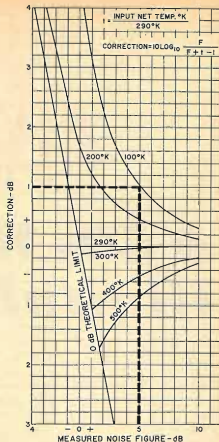
Fig. 3. Measurement errors are greater at the lower noise figure values. This graph is used when the input network behaves as though it were operating at other than 290° Kelvin. In the example, a 5-dB measurement is corrected to read 6 dB.
