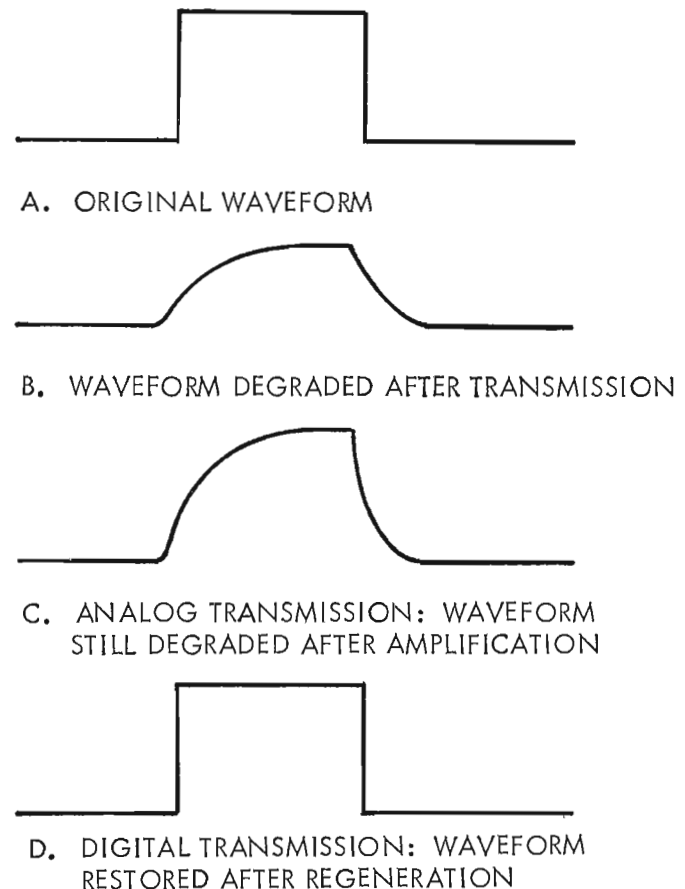
Fig. 1. During transmission, waveforms are degraded due to characteristics of the transmission media, but in a digital system, it's relatively easy to restore the original waveshape.
