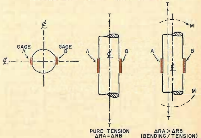
Fig. 6. If the test member is not loaded correctly (through its geometrical center), a bending moment can cause errors.
