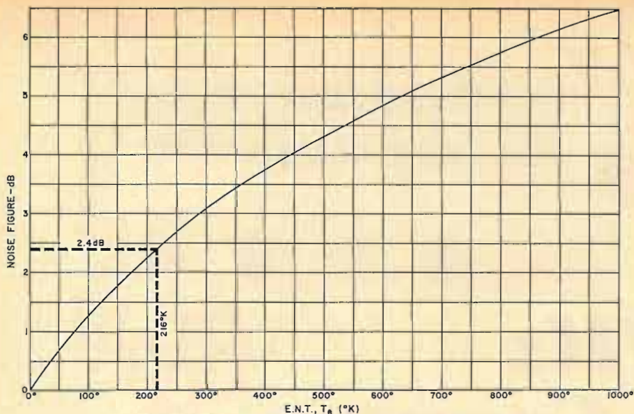
Fig. 2. This graph can be used to convert effective noise temperature measurements to their true noise figure value.
