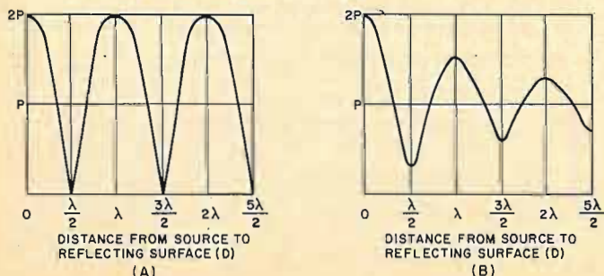
Fig. 3. When reflecting surface is much less than half a wavelength behind speaker, pressure of the sound at distant point approaches twice that of the loudspeaker alone.
