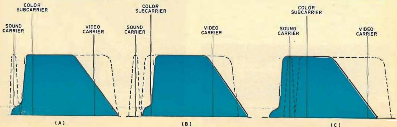
Fig. 1. The dashed curves represent the heterodyne output of the TV set converter stage. The heavy solid curves represent the set's i.f. bandpass response. (A) shows conditions with the fine-tuning control set at the proper position. Note that the video carrier is halfway down the slope of the i.f. response as required for proper equalization of the vestigial sideband transmission. In many cases, the color subcarrier is positioned halfway down the other side of the i.f. curve, rather as shown. In such a case, equalization is accomplished in the chroma section of the receiver. As the
